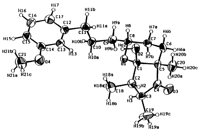
Figure 2. X-Ray Analysis diagram of (+)-5
