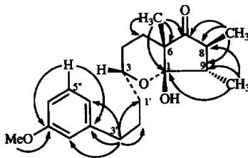
Figure 1. Major HMBC correlations for (+)- 5
